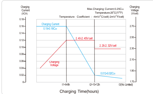
Charging Profile
